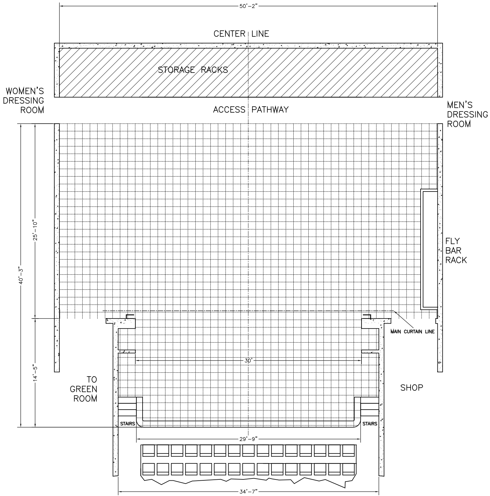
WDL STAGE LAYOUT (GRID SPACING = 1 FOOT SQUARE)
